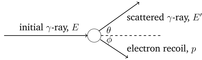
FIGURE 1. Compton scattering of \gamma -ray by an electron; E, E' are the particle energies, p the recoil momentum of the electron.
