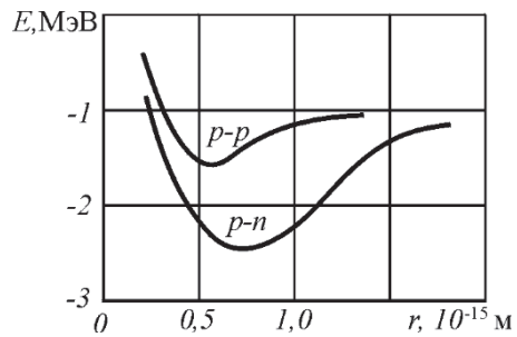
Fig. 6.6. Dependence of the interaction energy between nucleons (proton-proton and proton-neutron interactions) on the distance between them at antiparallel spins
