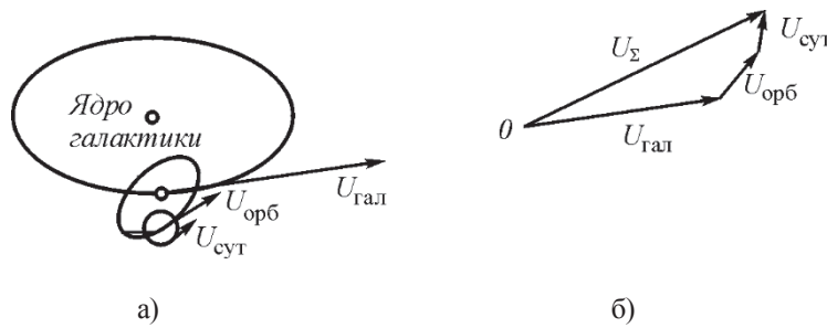
Fig. 9.12. Motion of a point located on the Earth's surface: a - galactic, orbital and daily velocities; б - vector summation of velocities
