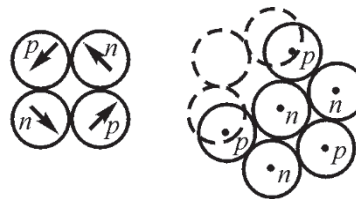
Fig. 6.18. Structure of core ^{10}_5\text{B}
