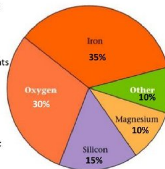
Bulk Earth composition
