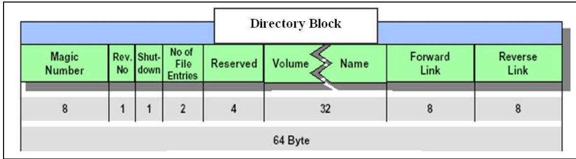
Figure 10-10. Directory Block
