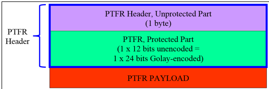
Figure 7-19. PT Data Frame Structure
