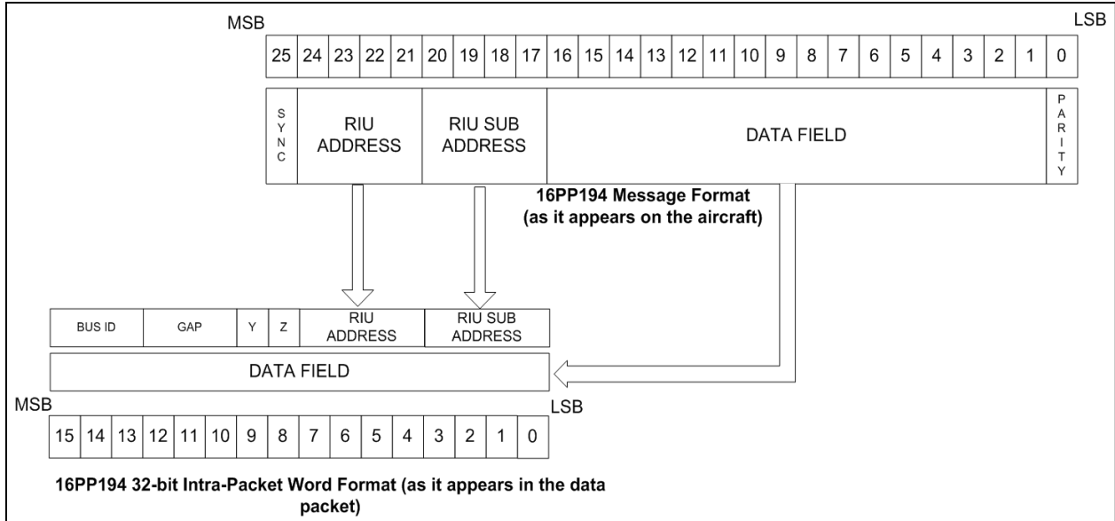
Figure 11-25. 16PP194 Word Format
