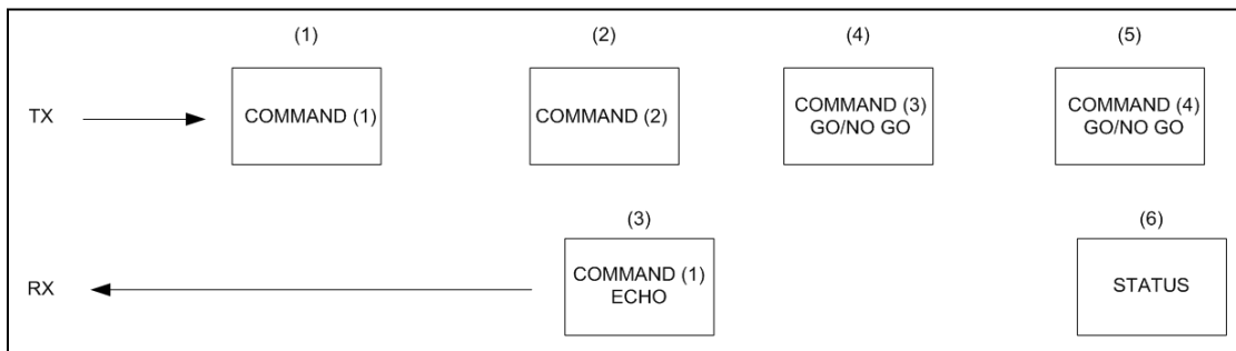
Figure 11-21. 16PP194 Message Transaction
