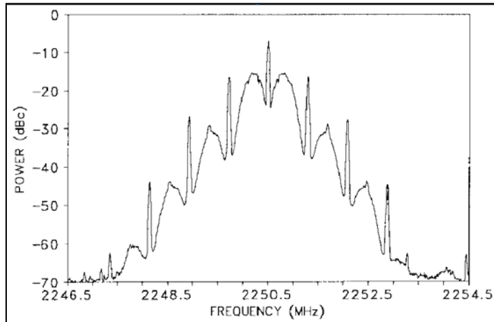
Figure A-6. Biφ PCM/PM Signal
