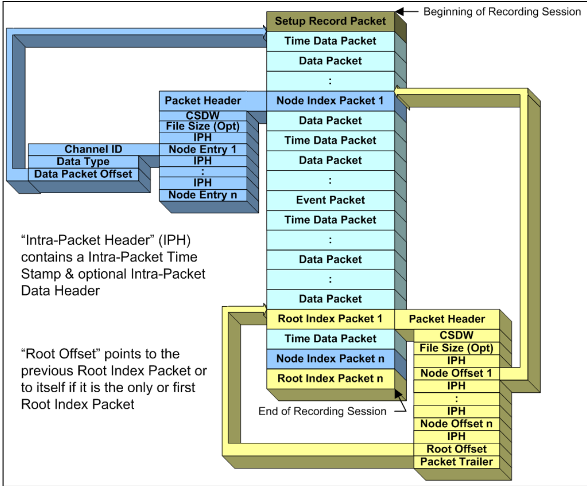
Figure 11-36. Format Showing Root Index Packet
